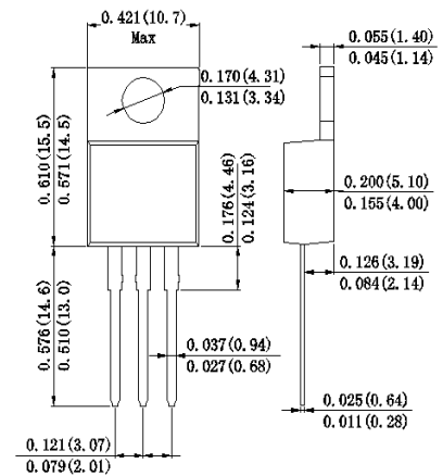
TO-220AB
